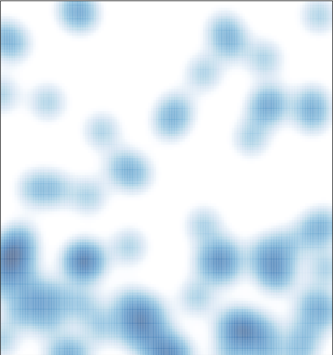
# features = 81 , max = 2
